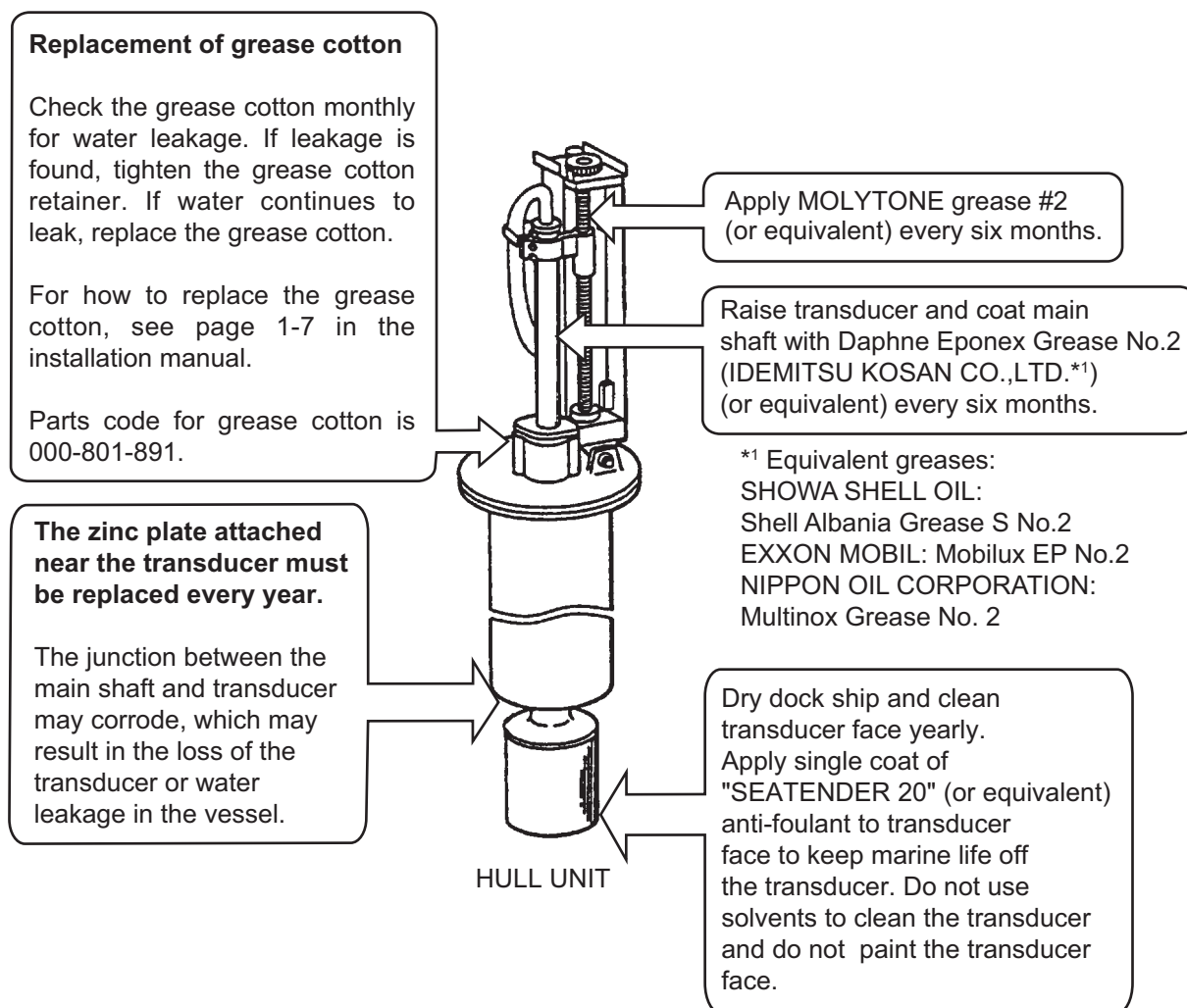
Hull unit maintenance points
