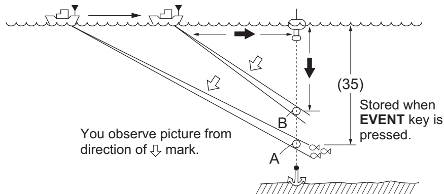
How to use the event mark
