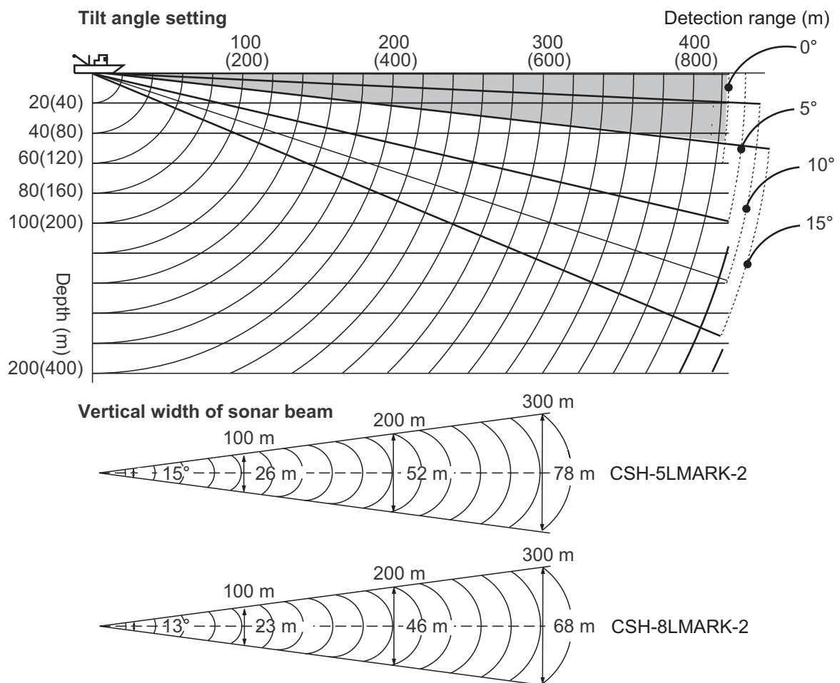
Depth, detection range and tilt angle
