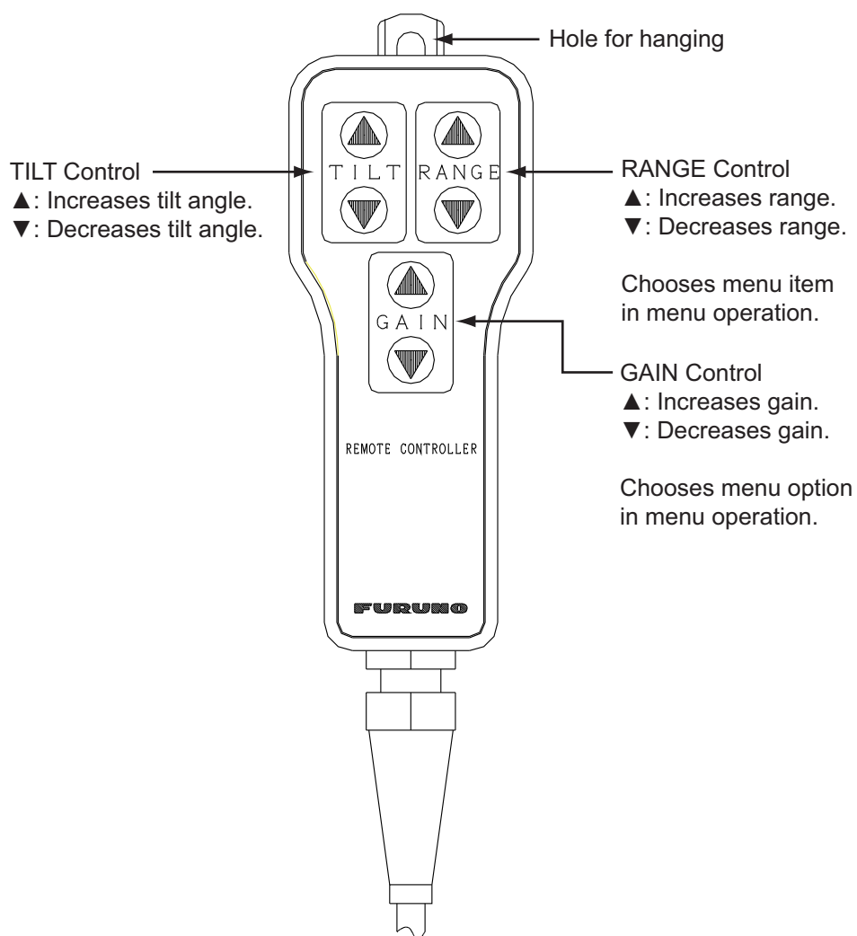
Remote controller
